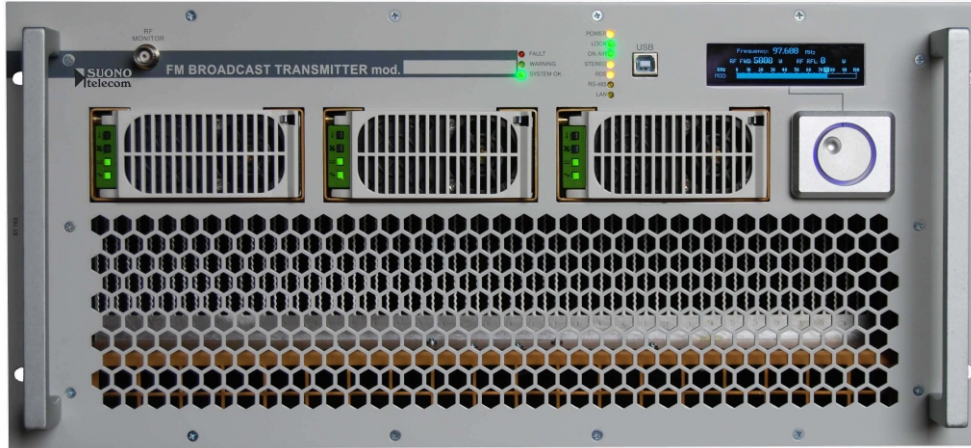
Frontplane (in threephase configuration)
